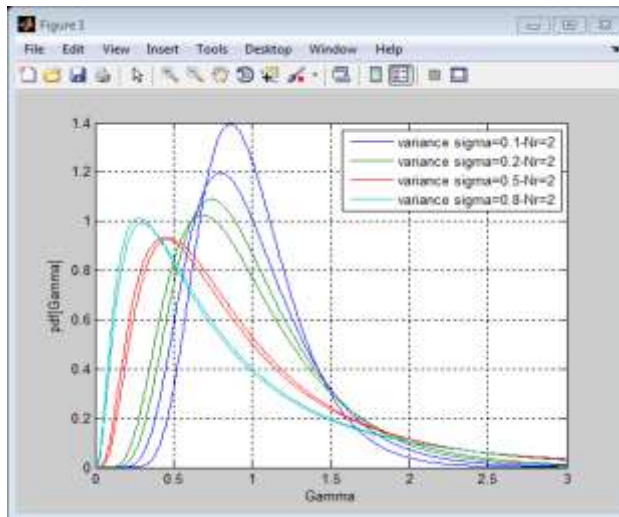
Figure 6 : Noise Variation
